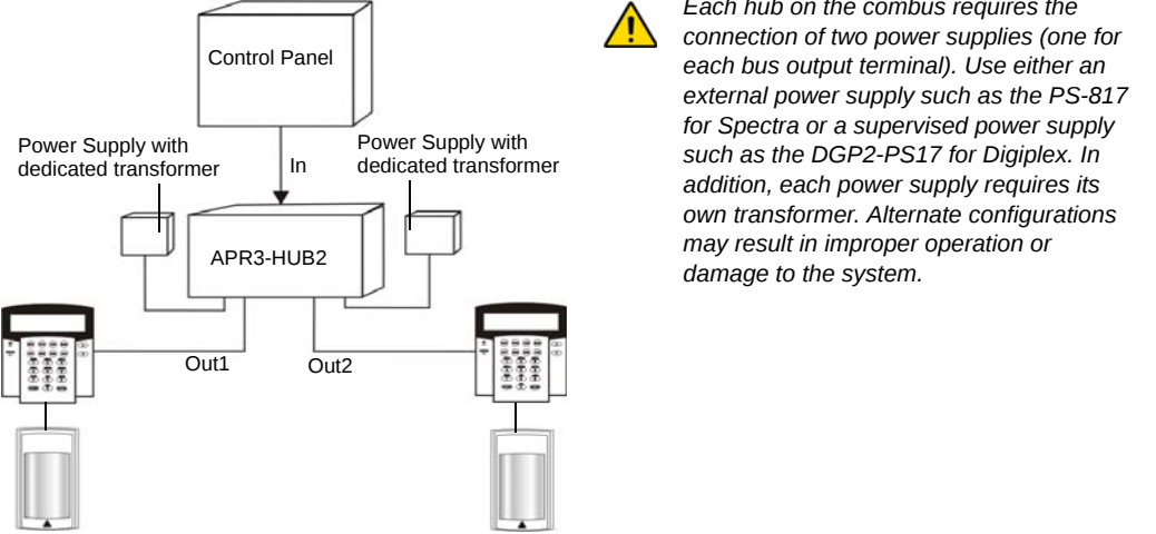
Figure 1 : Overview of the APR3-HUB2
