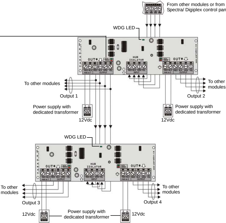
Figure 2 : Connecting the APR3-HUB2
