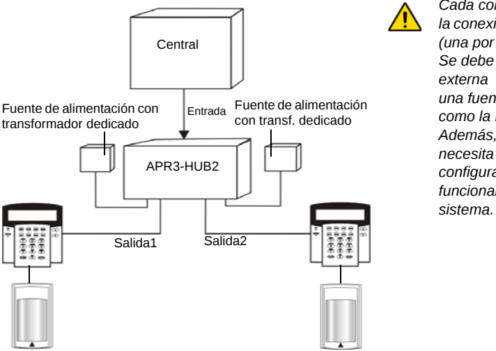
Figure 1 : Vista General del APR3-HUB2
